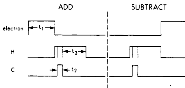
Figure 5. Pulse sequence for DNP-enhanced CPMAS ^{13}\text{C} NMR spectroscopy. Microwave pumping occurs during t_1 , cross-polarization during t_2 , and ^{13}\text{C} acquisition with H-C dipolar decoupling and magic-angle spinning occurs during t_3 . One block of the add-subtract, equal-heat, alternate-block sequence has the microwave irradiation after data acquisition has been completed. Relaxation effects during the two halves are equalized by inserting a t_1 delay at the end of the first half. Ordinary CPMAS ^{13}\text{C} NMR signals cancel exactly, so any difference signal obtained is from carbons coupled to electrons via the protons.
