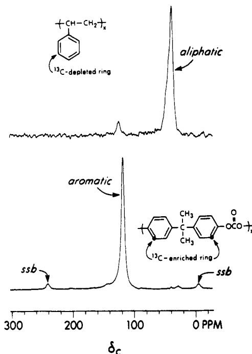
Figure 10. 15.1-MHz CPMAS ^{13}\text{C} NMR spectra of ^{12}\text{C} -enriched (99.97 atom %) polystyrene, PS( ^{12}\text{C} ) (top), and ^{13}\text{C} -enriched (99 atom %) polycarbonate, PC( ^{13}\text{C} ) (bottom). A total of 15 000 and 2760 scans were averaged to generate the PS and PC CPMAS spectra, respectively. Matched spin-lock transfers were made in 1.0 ms at 40 kHz; 80-kHz dipolar-decoupling fields were used. Spinning sidebands are designated "ssb".
