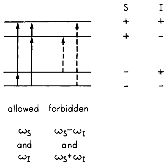
Figure 1. Energy-level diagram of uncoupled electron (S) and nuclear (I) spins in a strong external magnetic field. The solid lines indicate the ESR ( \omega_S ) and NMR ( \omega_I ) transitions corresponding to \Delta m = \pm 1 ; these are allowed transitions. The dashed lines indicate the zeroth-order "forbidden" transitions corresponding to \Delta m = 0, \pm 2 . The four energy levels are labeled by M_S, M_I .
