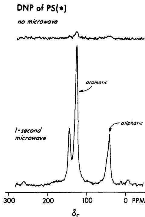
Figure 9. 15.1-MHz CPMAS ^{13}\text{C} NMR spectra of BDPA-doped polystyrene with (bottom) and without (top) 1.0-s microwave irradiation at the difference of the electron and proton Larmor frequencies. The microwave irradiation produces a positive DNP enhancement. The peak around \delta_{\text{C}} 40 is from the aliphatic carbons, the peak around \delta_{\text{C}} 125 is from all protonated, aromatic carbons, and the peak around \delta_{\text{C}} 145 is from the nonprotonated aromatic carbon.
