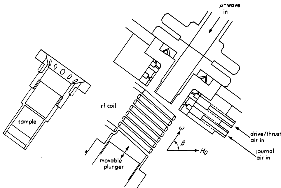
Figure 4. Rotor, stator, radio-frequency (rf) coil, and waveguide configuration of the DNP CPMAS ^{13}\text{C} NMR spectrometer. Remote rf tuning elements are connected to the coil by a transmission line (not shown in the figure). The movable plunger (reflector) is pneumatically operated and together with the rf coil makes up the microwave cavity. The magic angle, \beta , is 54.7^\circ .
