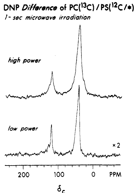
Figure 14. 15.1-MHz CPMAS ^{13}\text{C} NMR DNP difference spectra of the thin-film PC( ^{13}\text{C} )/PS( ^{12}\text{C}/* ) blend. Increasing microwave power increases the difference signal intensity but broadens the lines (top spectrum) because of contributions from carbons that are close to the free-radical centers. In both cases 1.0-s microwave irradiation was used. The spectrum at the top of the figure is an expanded version of the spectrum shown in Figure 12 (top).
