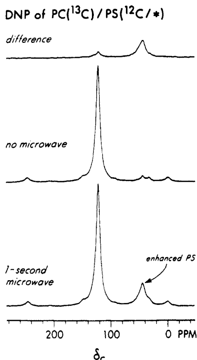
Figure 12. 15.1-MHz CPMAS ^{13}\text{C} NMR spectra of PC( ^{13}\text{C} )/PS( ^{12}\text{C}/* ) with (bottom) and without (middle) 1.0-s microwave irradiation. The difference spectrum (top) has a polycarbonate contribution ( \delta_c 120) arising from PC chains at the interface. Each spectrum was generated by 72 000 scans with a 1.0-s recycle period.
