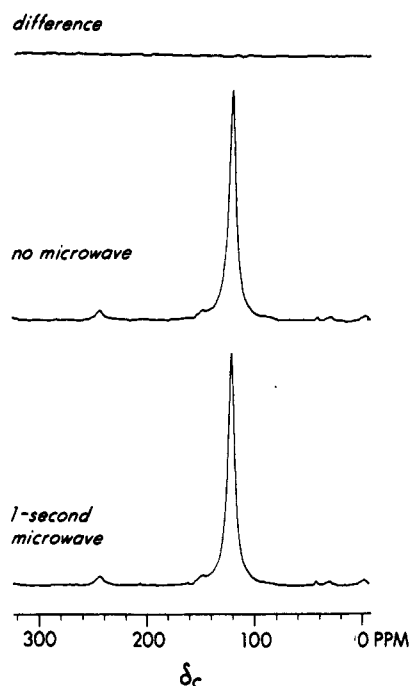
Figure 11. 15.1-MHz CPMAS ^{13}\text{C} NMR spectra of PC( ^{13}\text{C} ) with (bottom) and without (middle) 1.0-s microwave irradiation. A total of 2475 scans were averaged to obtain each spectrum. The null spectrum shown at the top is the difference (bottom minus middle).
