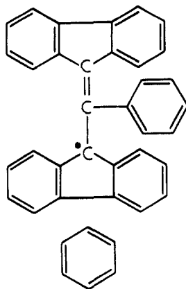
Figure 6. Structure of 1,3-bis(diphenylene)-2-phenylallyl (BDPA) free-radical complex with benzene.
