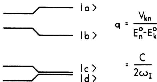
Figure 2. Energy-level diagram of an electron and nuclear spin pair with dipolar coupling. The spin states are identified in eq 7 of the text.
