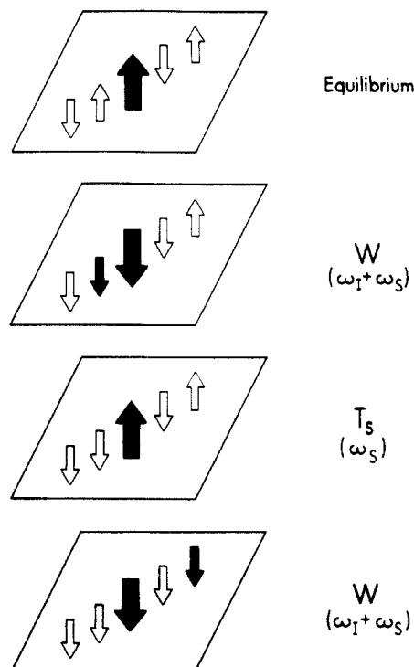
Figure 3. Single electron (big arrow) shown dipolar coupled to many isolated nuclei (small arrows). Irradiation at the sum of the electron (S) and nuclear (I) Larmor frequencies induces "forbidden" double-quantum transitions leading to a negative DNP enhancement. The electron spin-lattice relaxation time ( T_S ) is short while the nuclear spin-lattice relaxation times ( T_I ) are long. Thus, a single electron can polarize many nuclei under microwave pumping. Irradiation at the difference of the electron and nuclear Larmor frequencies produces a positive DNP enhancement by inducing "forbidden" zero-quantum, flip-flop transitions.
