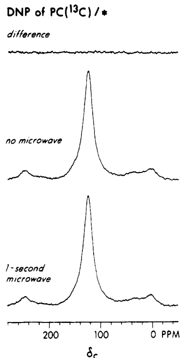
Figure 13. 15.1-MHz CPMAS ^{13}\text{C} NMR spectra of a thin film of PC( ^{13}\text{C} )/*. A thin-film of PC( ^{13}\text{C} ) on a microscope glass slide was dipped in a cyclohexane solution of BDPA at 38 °C (with no polystyrene present in the cyclohexane solution) and then dried. The BDPA crystallized on the surface of the polycarbonate film. The line width increase is due to bulk-susceptibility broadening. The spectra were obtained by a CPMAS ^{13}\text{C} NMR spectrometer with (bottom) and without (middle) 1.0-s microwave irradiation. About 5000 scans were averaged to obtain each spectrum. The difference spectrum is shown at the top of the figure, a null indicating that the BDPA has not penetrated the chains of polycarbonate.
