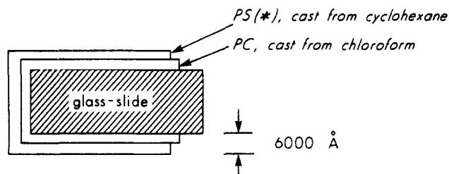
Figure 8. Preparation of a thin film of polycarbonate-polystyrene blend by double casting. The PC was cast from chloroform solution at room temperature and the PS with BDPA from a solution of cyclohexane at 38 °C. The asterisk within parentheses indicates the presence of homogeneously-dispersed free radicals in the PS phase.
