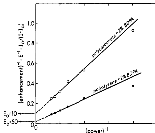
Figure 7. Inverse of the proton-observed DNP enhancements in PS(*) and PC(*) as a function of the inverse of the relative microwave-irradiation power. The inverse enhancements are expressed as I_0/(I - I_0) , where I is the integrated intensity of the solid-echo signal with microwave irradiation and I_0 is that without microwave irradiation (part 2). The enhancements at infinite microwave power are obtained by extrapolation.
